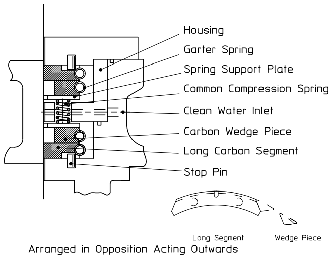
Fig. 4 Wedge-type gland rings
