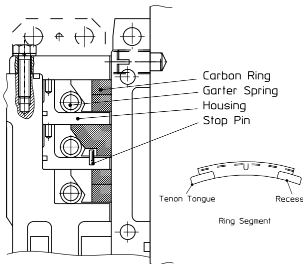
Fig. 2 Tenon-type gland
