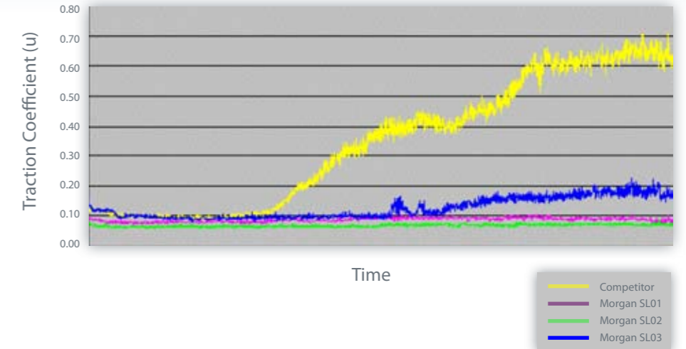
Comparitive results showing Traction Coefficient Vs Time
