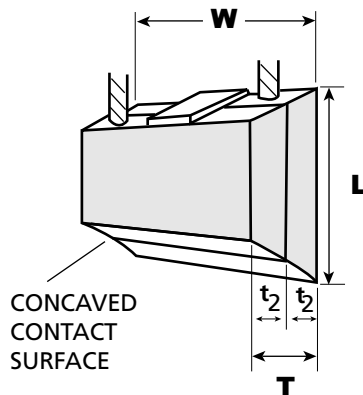
Figure 4. Multi-wafer Brush
