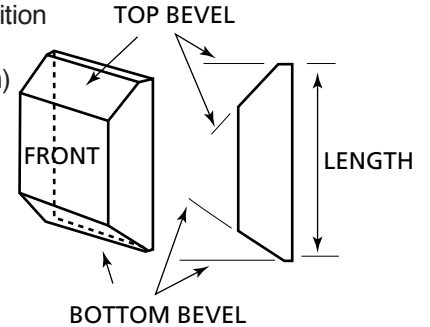
Figure 6. Bevels
