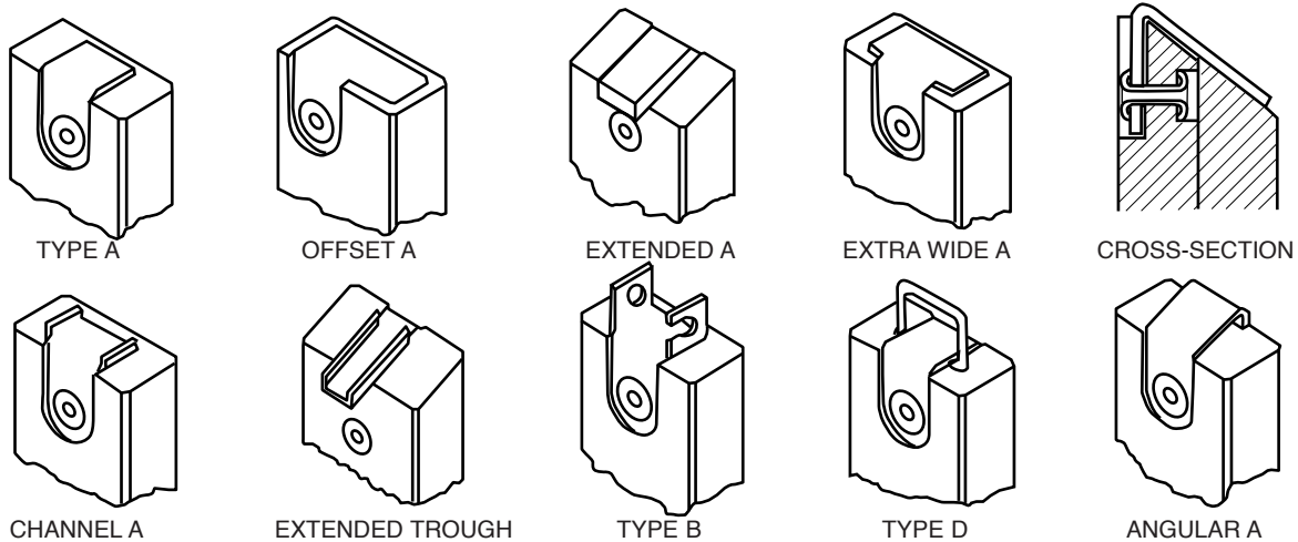
Figure 17. Clips
