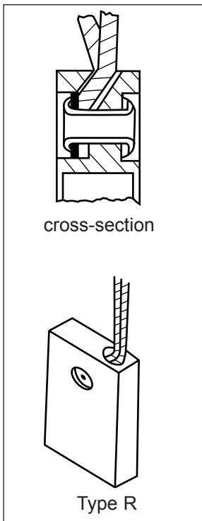
Figure 12. Rivet Connections
