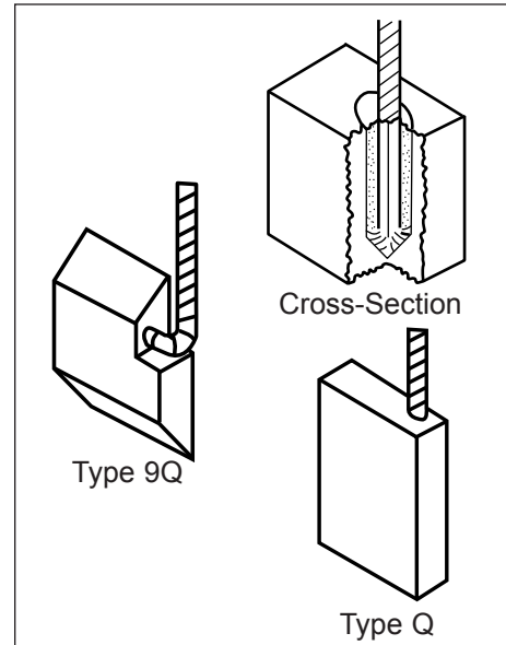
Figure 11. Tamped Connections
