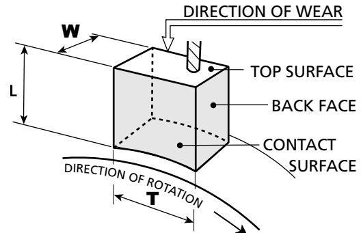
Figure 2. Slip Ring Brush
