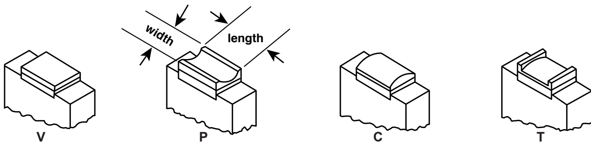
Figure 16. Pad Styles
