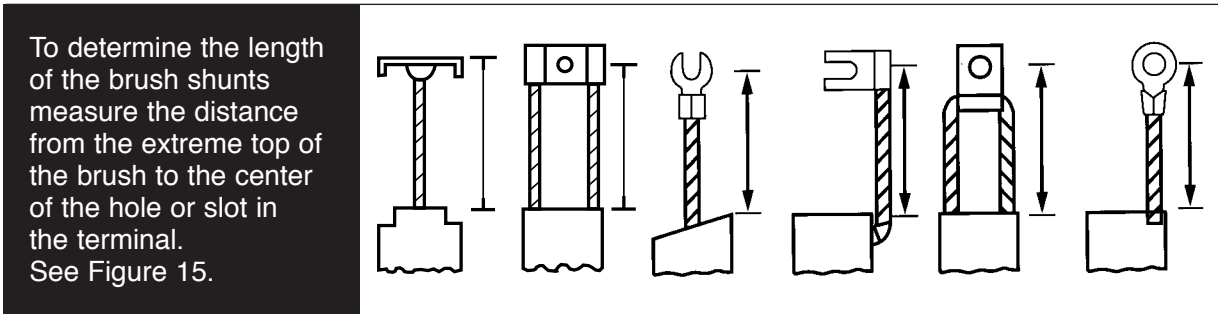
Figure 15. Shunt Length
