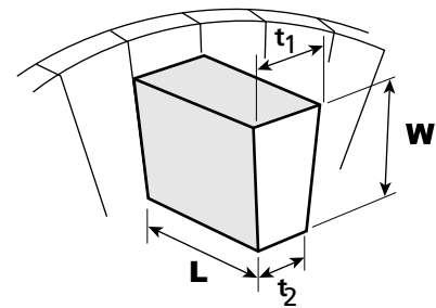
Figure 5. Wedge Brush
