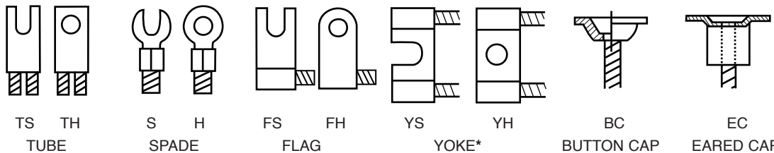
Figure 18. Terminals
