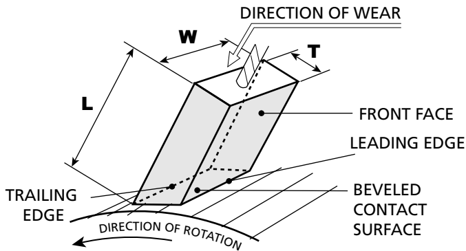
Figure 1. Commutator Brush
